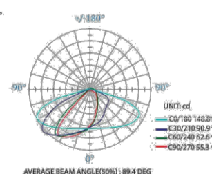
INTENSITY DISTRIBUTION DIAGRAM IN C PLANS
