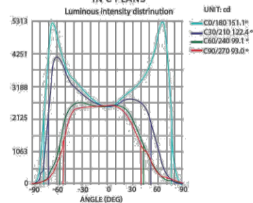
INTENSITY DISTRIBUTION DIAGRAM IN C PLANS
